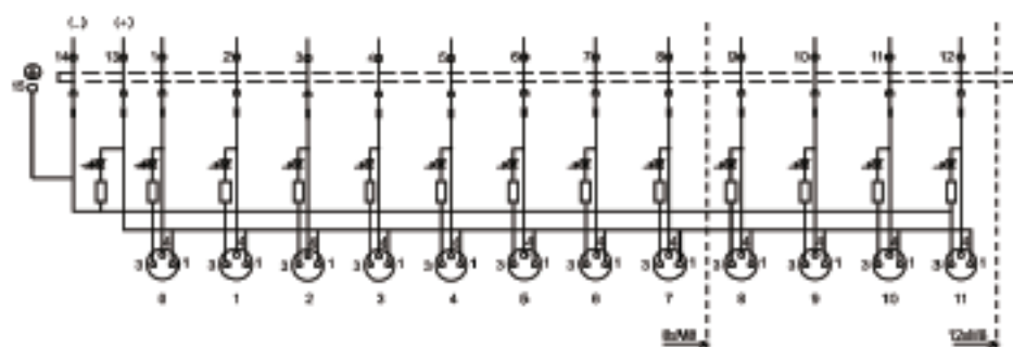
PNP
