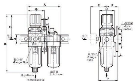
DAC3010~5010
