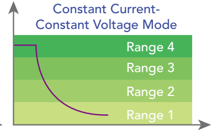
Multi-Current Range
