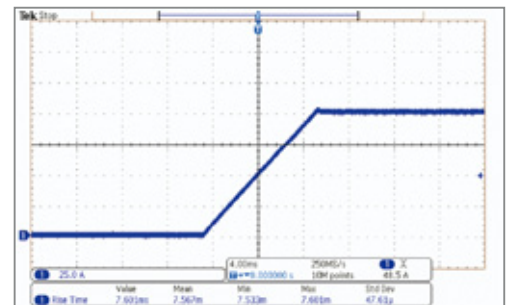
Rise Time<10mS
